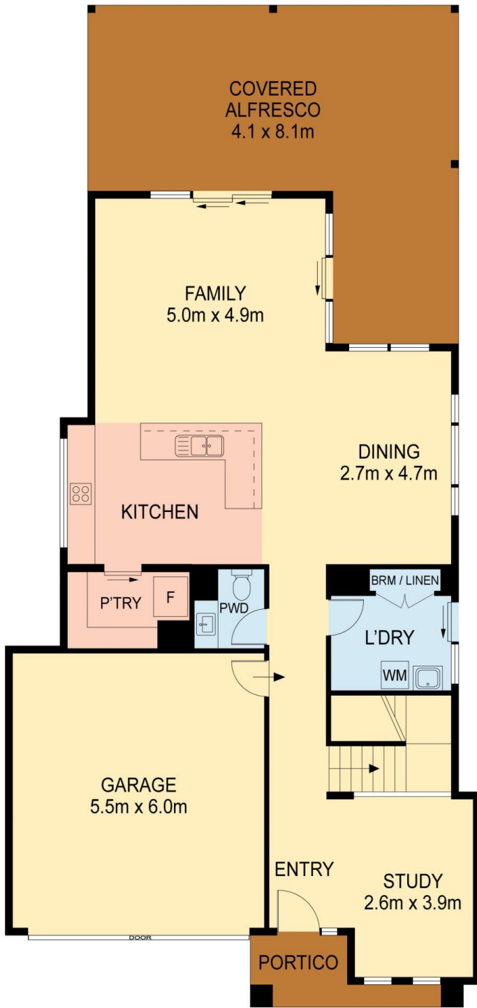
GROUND FLOOR
